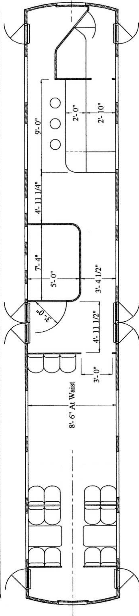
57'-0" Over Corners
